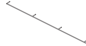
① METAL L4 1032x45.8 - 4PCS
